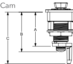
Lifter Cam
