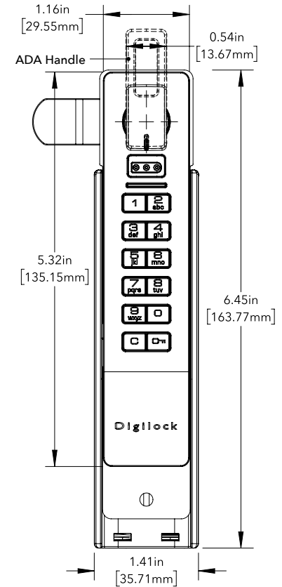
Slam Latch
