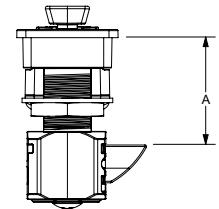
Slam Latch
